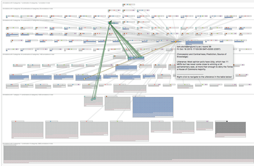
Figure 5.7: Example of a CatCombos visualization for the complete data set of about 10,000 text annotations. Here, the user has highlighted all annotations related to the category CONCESSION AND CONTRARINESS represented by blue dots using the filtering panel (see Figure 5.8 and Section 5.4.2). Yellow and green links connect the currently highlighted (by hovering) and pinned (by clicking) annotation items to other annotations made for the same utterances, respectively. Reprinted from [242] © 2017 ACM.
