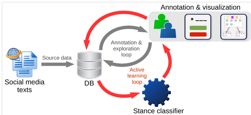
Figure 5.1: The overview of the main aspects of the proposed approach. The overall process involves the annotation and visual exploration loop initiated by the users (in gray), and the active learning loop initiated by the stance classifier (in red). Reprinted from [242] © 2017 ACM.
