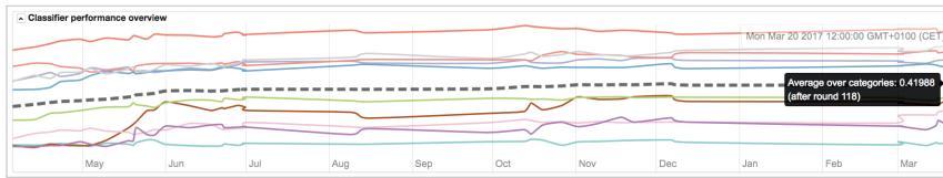
Figure 5.12: The historical classifier performance plot. The tooltip for the thick dashed line reveals the average value over all categories after the latest active learning round. Reprinted from [242] © 2017 ACM.
