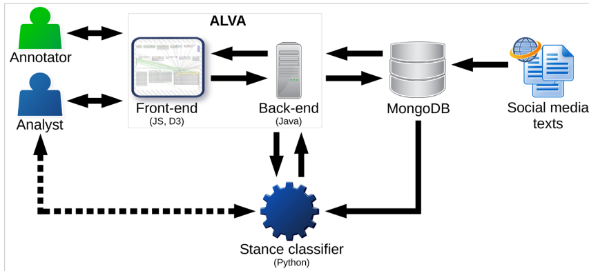
Figure 5.3: Architecture of ALVA. The dashed line indicates interaction between CL experts and the classifier, which is outside of the scope of our system presented in this chapter. Reprinted from [242] © 2017 ACM.
