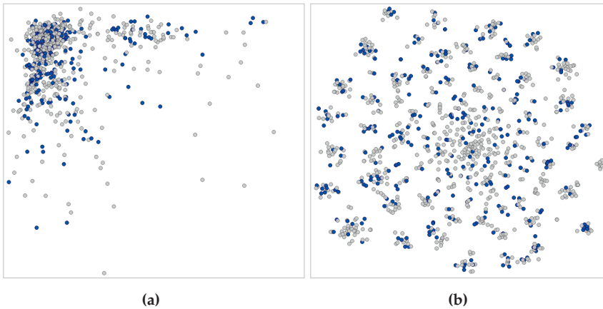
Figure 5.15: VSM visualizations in ALVA using (a) PCA (the first and second principal components) and (b) t-SNE projections. While the positions of visual items are based on the VSM model, the highlighting with blue color is applied to the stance category CONCESSION AND CONTRARINESS in the corresponding annotations. Reprinted from [242] © 2017 ACM.
