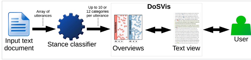
Figure 7.2: The architecture of our approach. DoSVis uses the output of the stance classifier for a text document divided into utterances. Each utterance may be simultaneously labeled with multiple stance categories. Reprinted from [239] © 2018 SciTePress.
