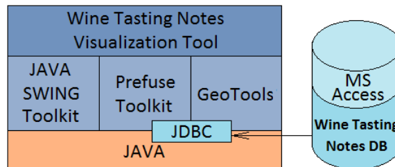
Fig. 5.11 Software architecture of the tool.
